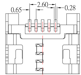
P.C.B LAYOUT MOUNTING PATTERN
