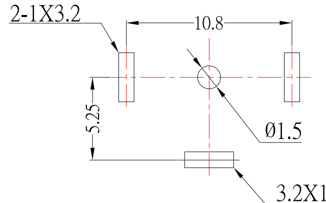
PCB HOLES DIAGRAM TOP VIEW
