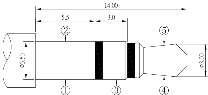
ø3.50mm 3 POLE PLUG
