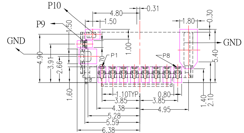
PCB LAYOYT
