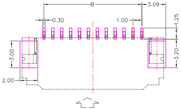
FPC/FFC Insert Direction
