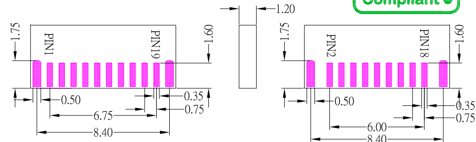
PCB LAYOUT
