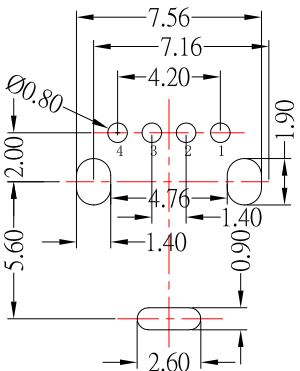
PCB LAYOUT
