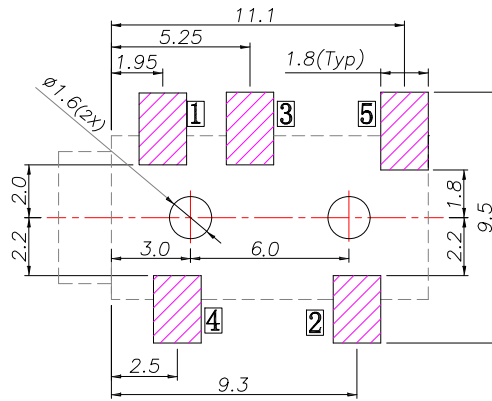
RECOMMENDED P. C. B. LAYOUT (COPPER-SIDED VIEW)
