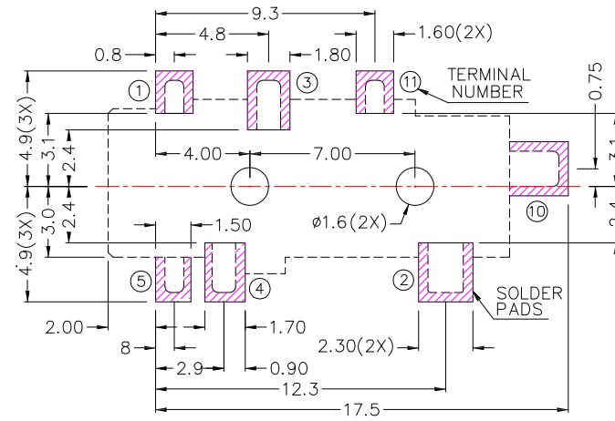
RECOMMENDED SOLDER PAD LAYOUT (TOP VIEW)
