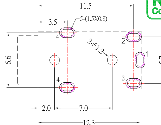
P.C.B LAYOUT MOUNTING PATTERN (TOP VIEW)
