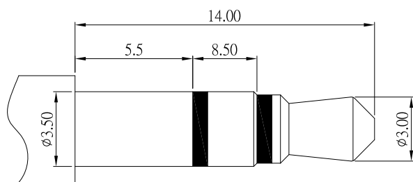
ø3.50mm 3 POLE PLUG
