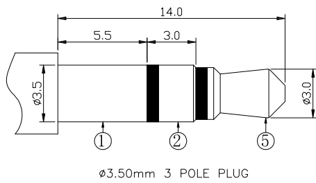
Ø3.50mm 3 POLE PLUG
