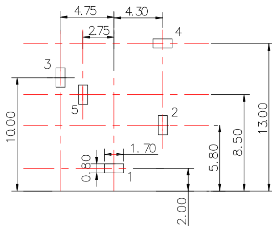
PCB LAYOUT
