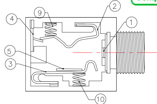
Internal construction
