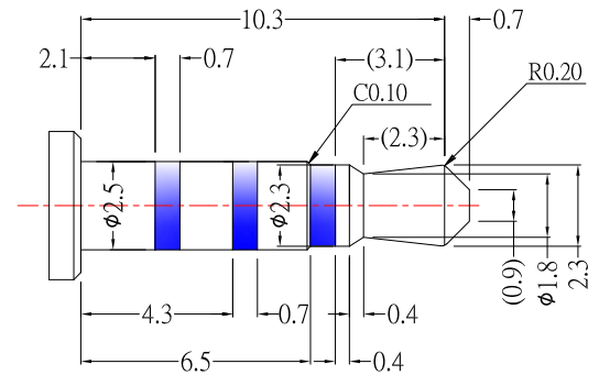
ø2.50mm 4 POLE PLUG DETAIL DRAWING
