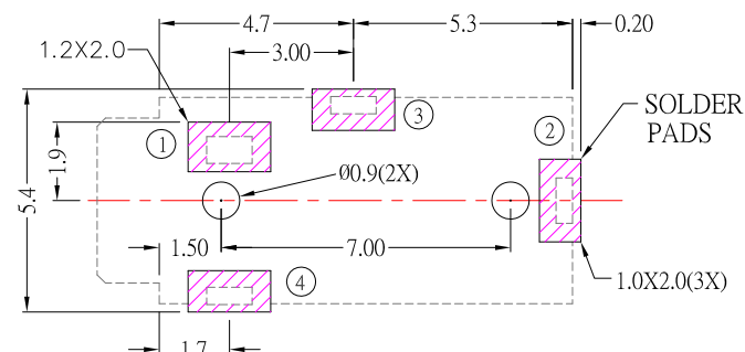
RECOMMENDED SOLDER PAD LAYOUT
