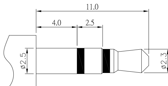
Ø2.50mm 3 POLE PLUG
