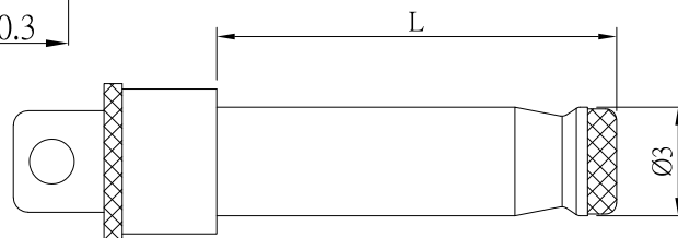
RECOMMENDED PLUG
