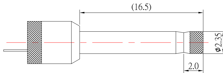
RECOMMENDED PLUG
