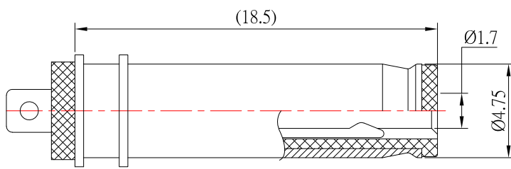
RECOMMENDED PLUG
