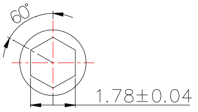
Shaft hole shape and dimension
