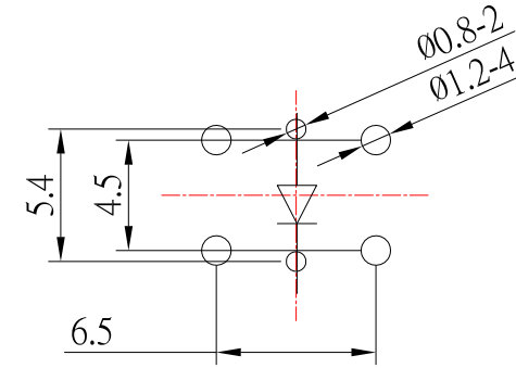
MOUNTING PATTERN
