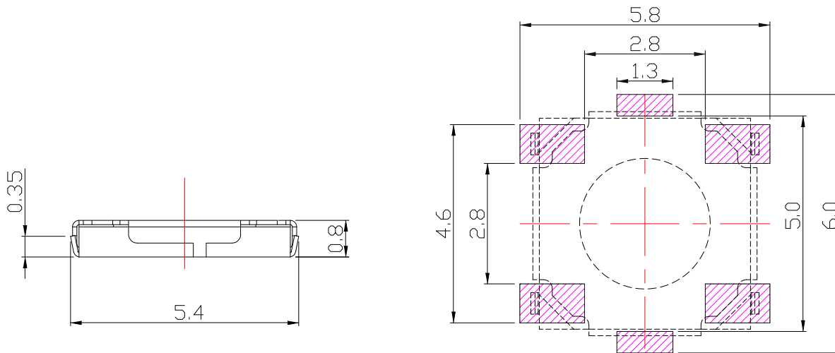
P.C.B. LAYOUT MOUNTING PATTERN
