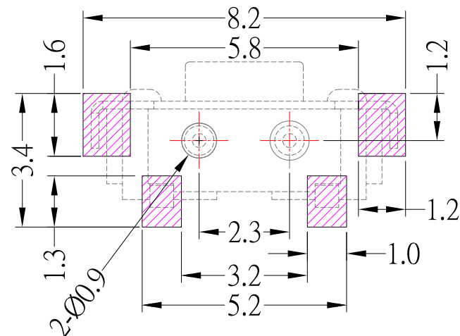
P.C.B MOUNTING PATTERN DIMENSION
