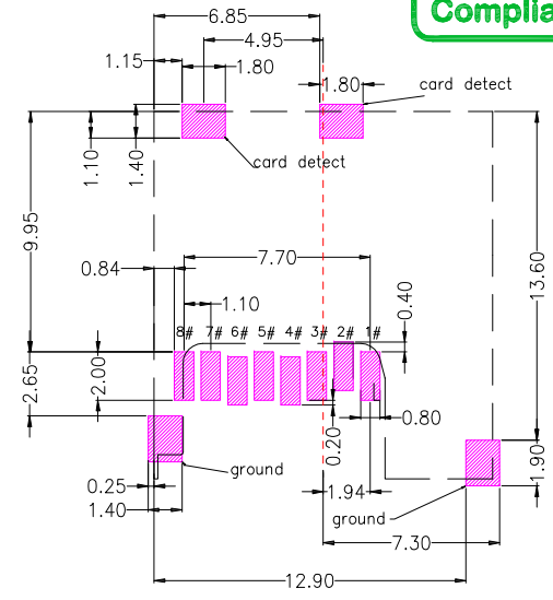
PCB LAYOYT
