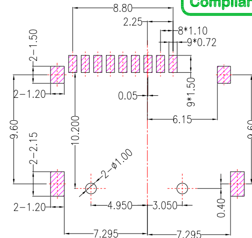
PCB LAYOYT
