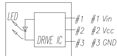
Internal equivalent circuit
