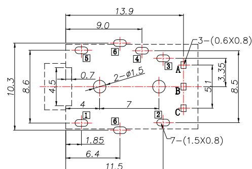
P.C.B LAYOUT MOUNTING PATTERN (COPPER-SIDED VIEW)
