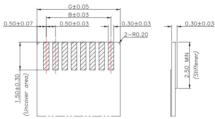
RECOMMENDED FPC/FFC DIMENSIONS
