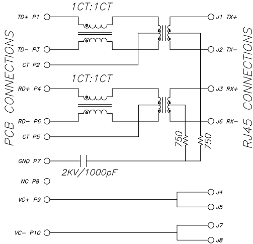
SCHEMATIC
