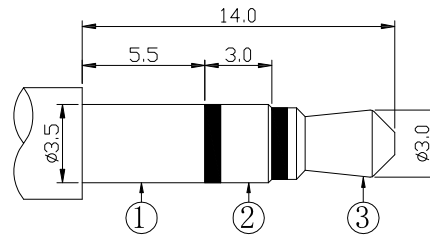
3.5mm 3 POLE PLUG
