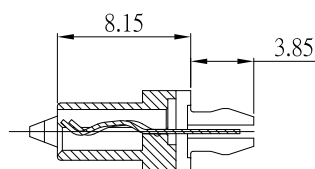
SECTION C-C
