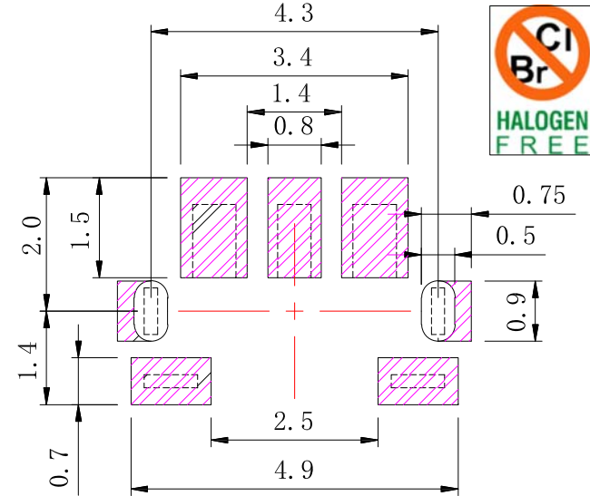
PCB LAYOUT
