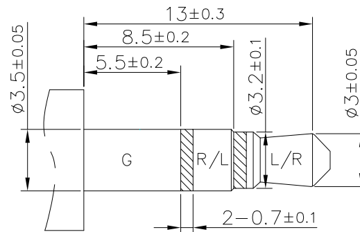
RECOMMENDED PLUG ø3.5 3-POLE STANDARD PLUG
