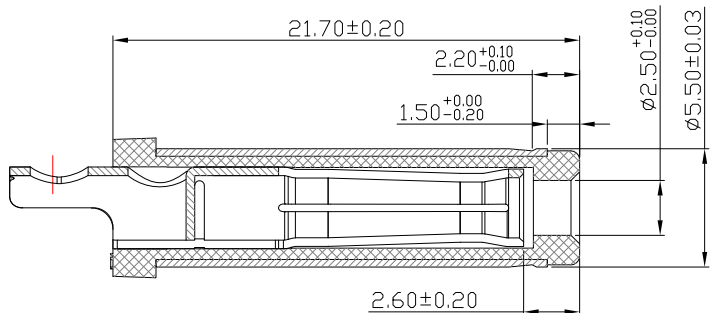
MATING PLUG
