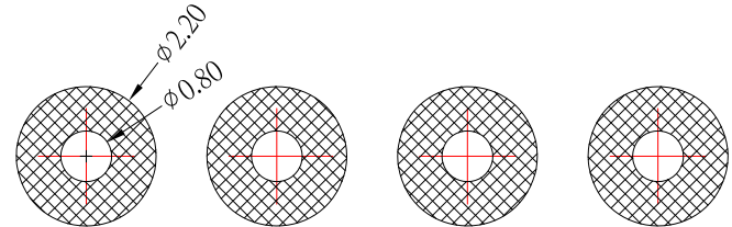
Recommend PCB Layout
