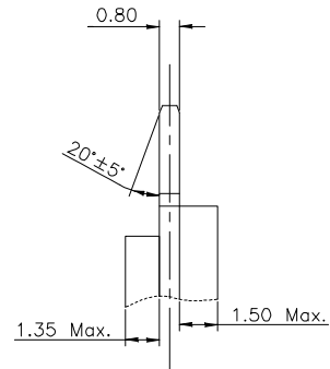
PLUG PCB
