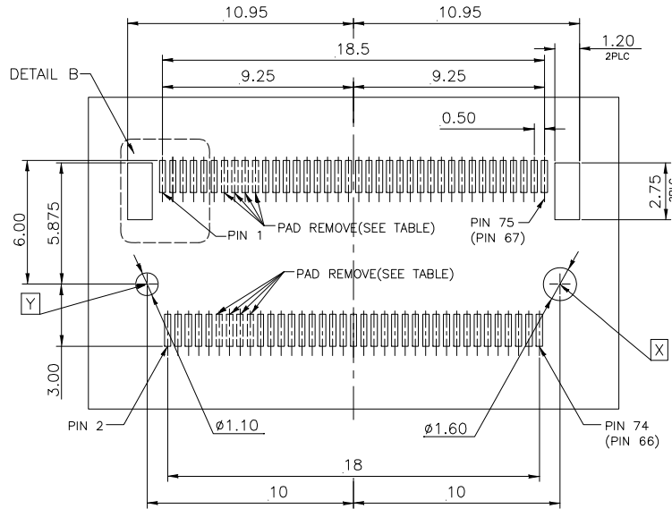
RECOMMEDNED NGFF MOUNTING TYP PCB_LAYOUT
