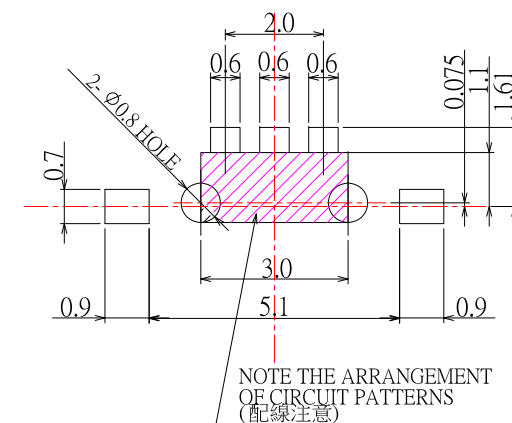
P.C.B MOUNTING PATTERN
