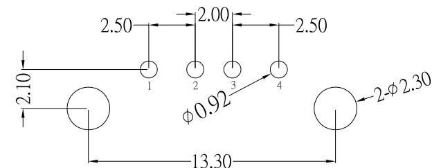
P.C.B LAYOUT MOUNTING PATTERN
