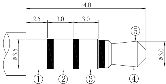
ø3.50mm 4 POLE PLUG
