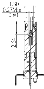
SECTION: B-B
