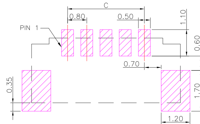
P.C.B LAYOUT MOUNTING PATTERN
