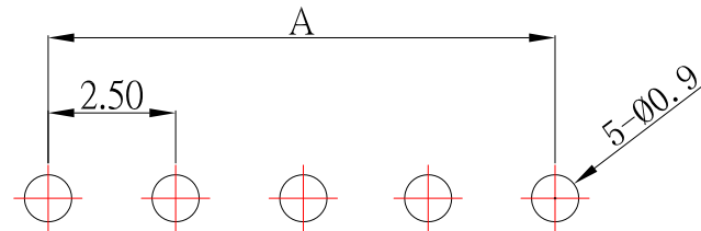
P.C.B LAYOUT MOUNTING PATTERN
