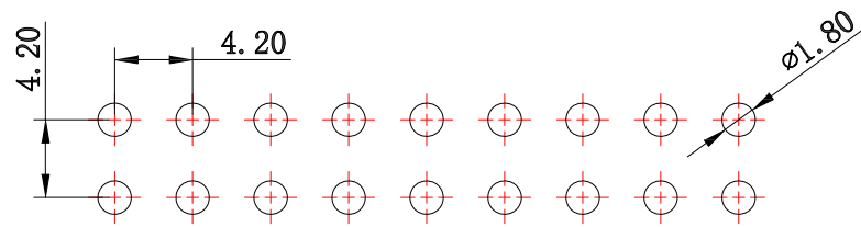
P.C.B LAYOUT MOUNTING PATTERN
