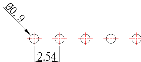
P.C.B LAYOUT MOUNTING PATTERN
