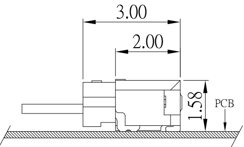
MATED CONDITION
