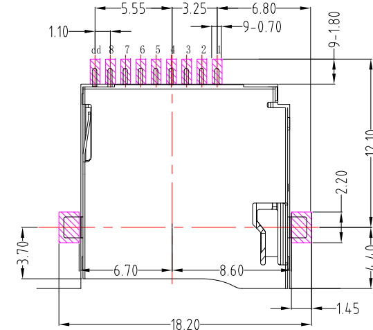
PCB LAYOYT
