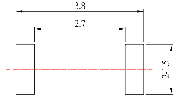
P.C.B LAYOUT MOUNTING PATTERN
