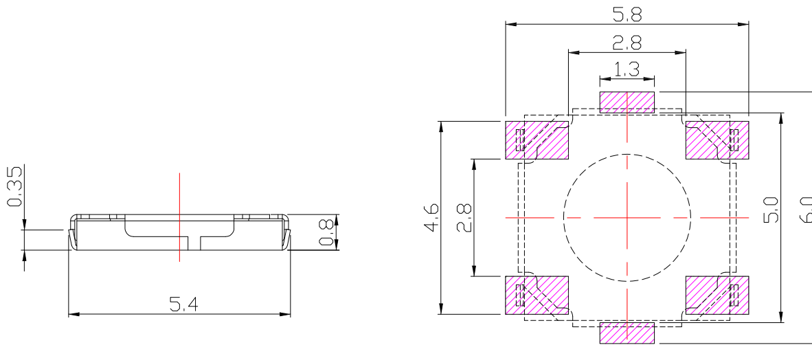
P.C.B. LAYOUT MOUNTING PATTERN
