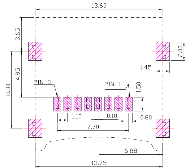
PCB LAYOYT
