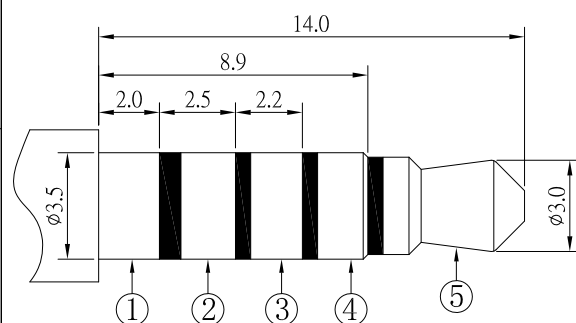
ø3.50mm 5 POLE PLUG
